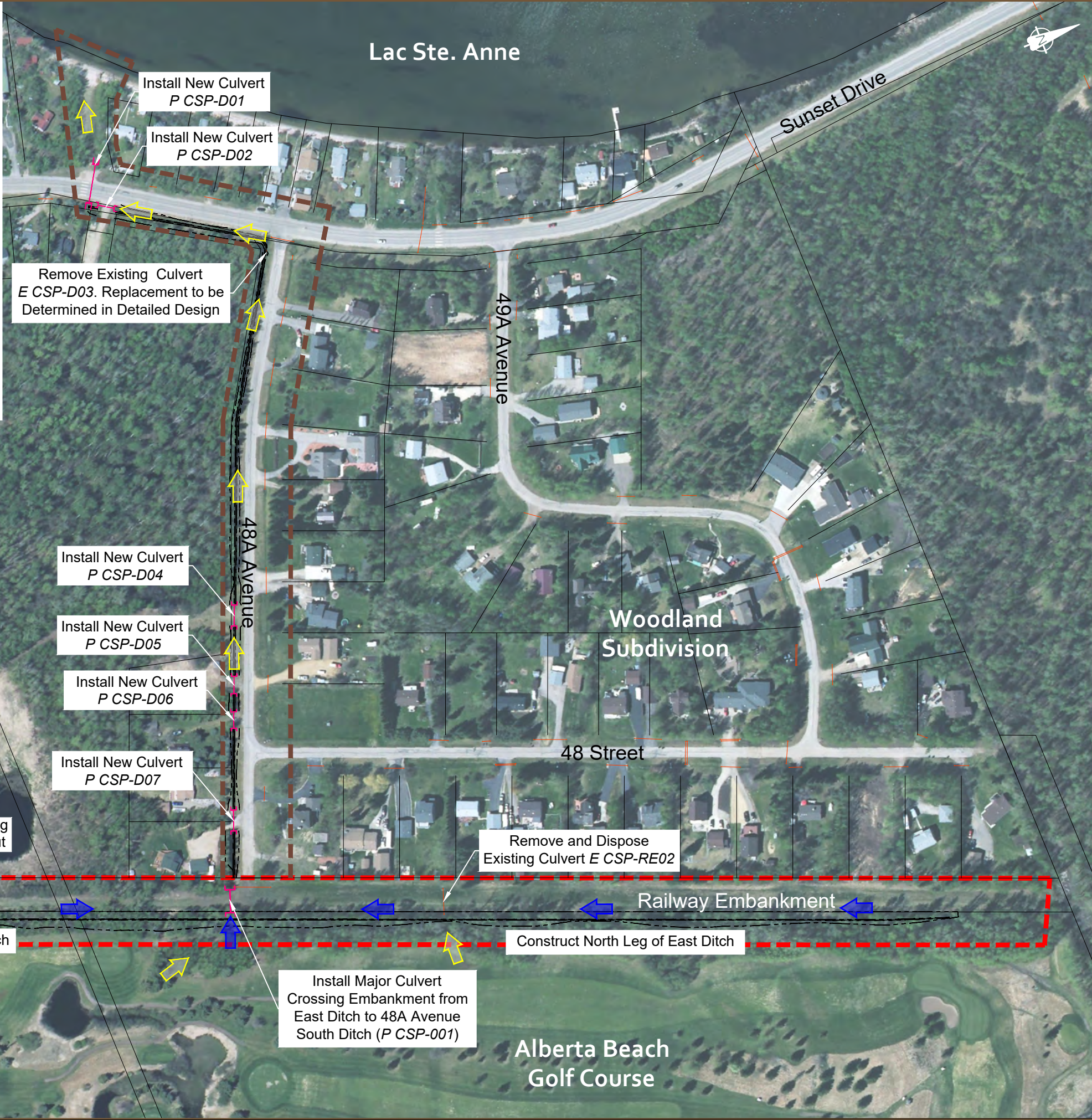
Figure 10 Project 1: Embankment Drainage System
