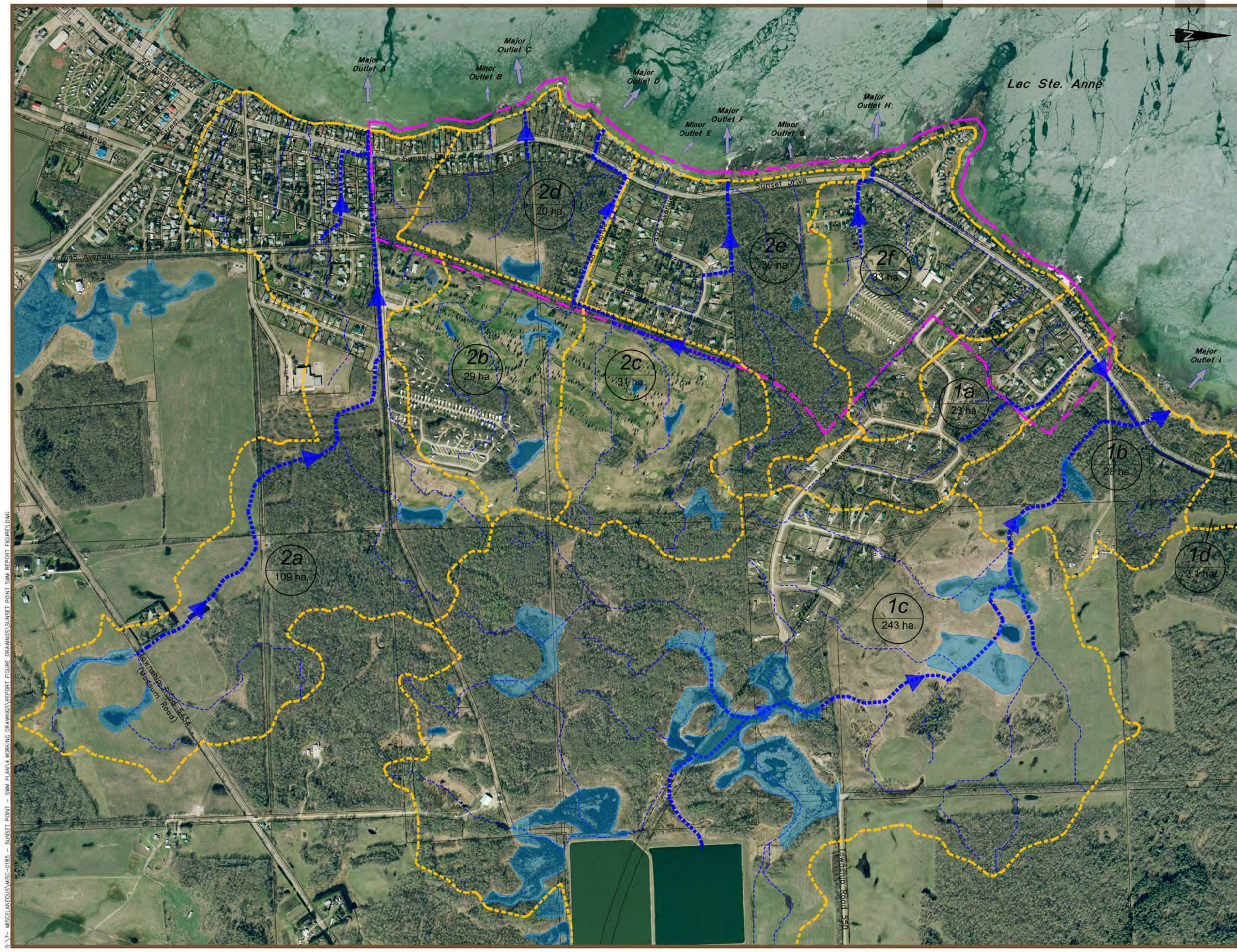
Figure 6 Existing Drainage Features
