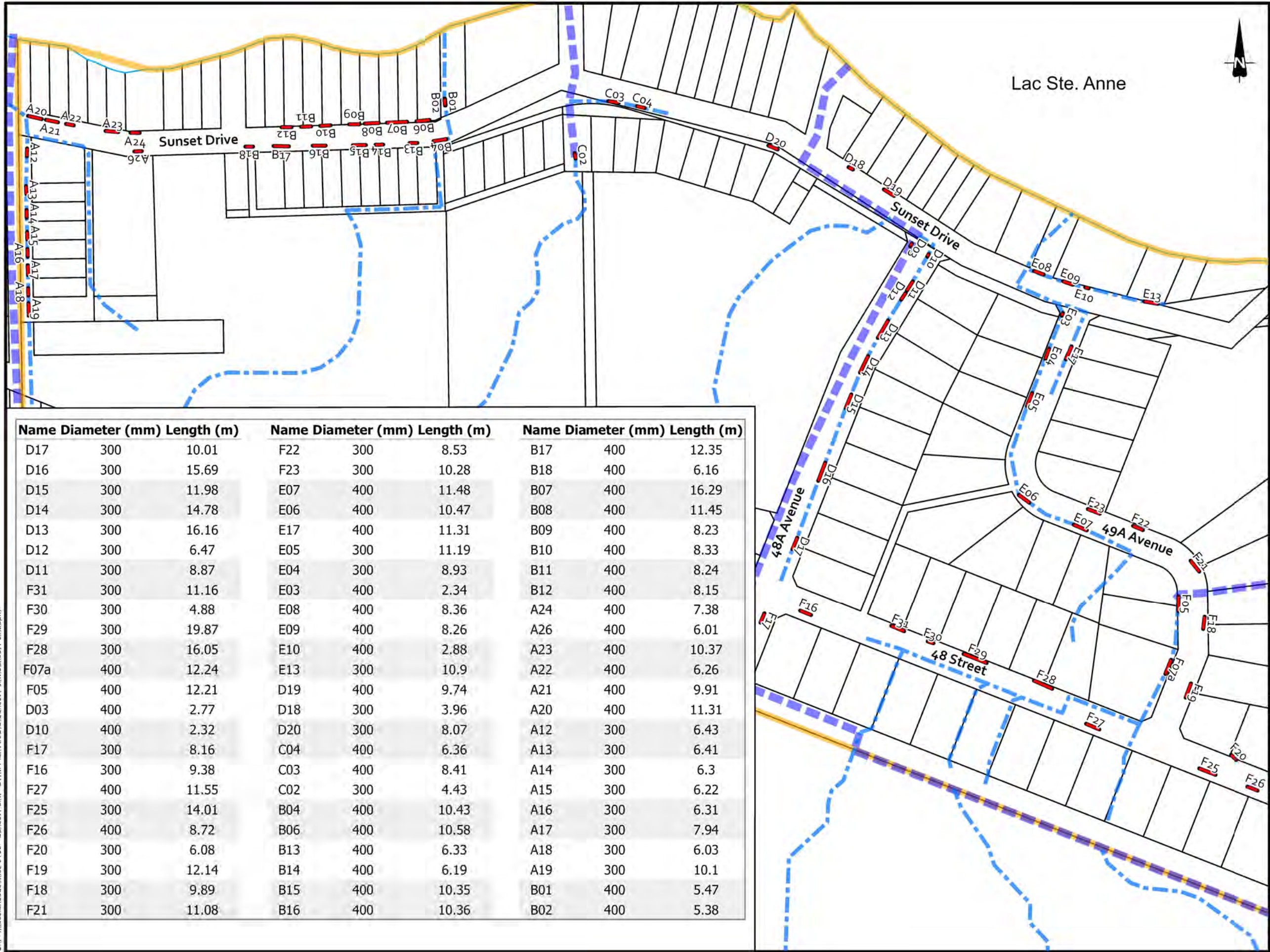
Figure 16 Undersized Culverts - 1/2
