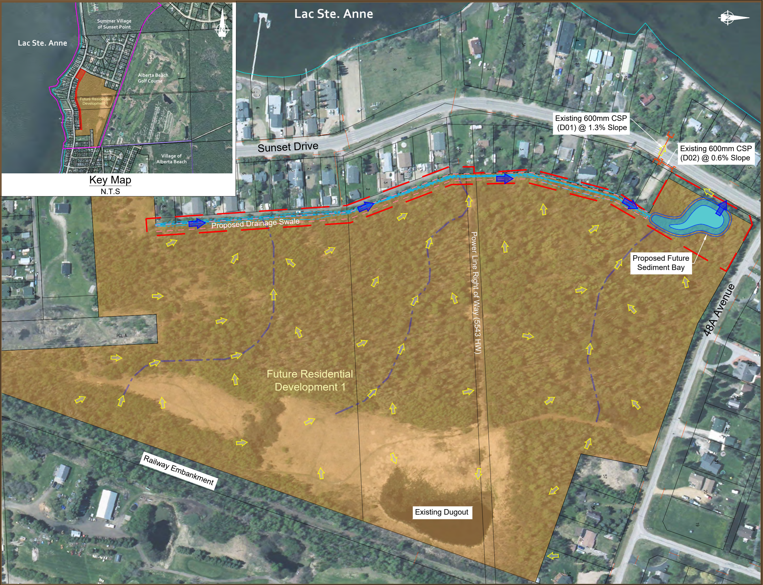
Figure 14 Drainage Recommendations for Future Residential Development Parcel 1
