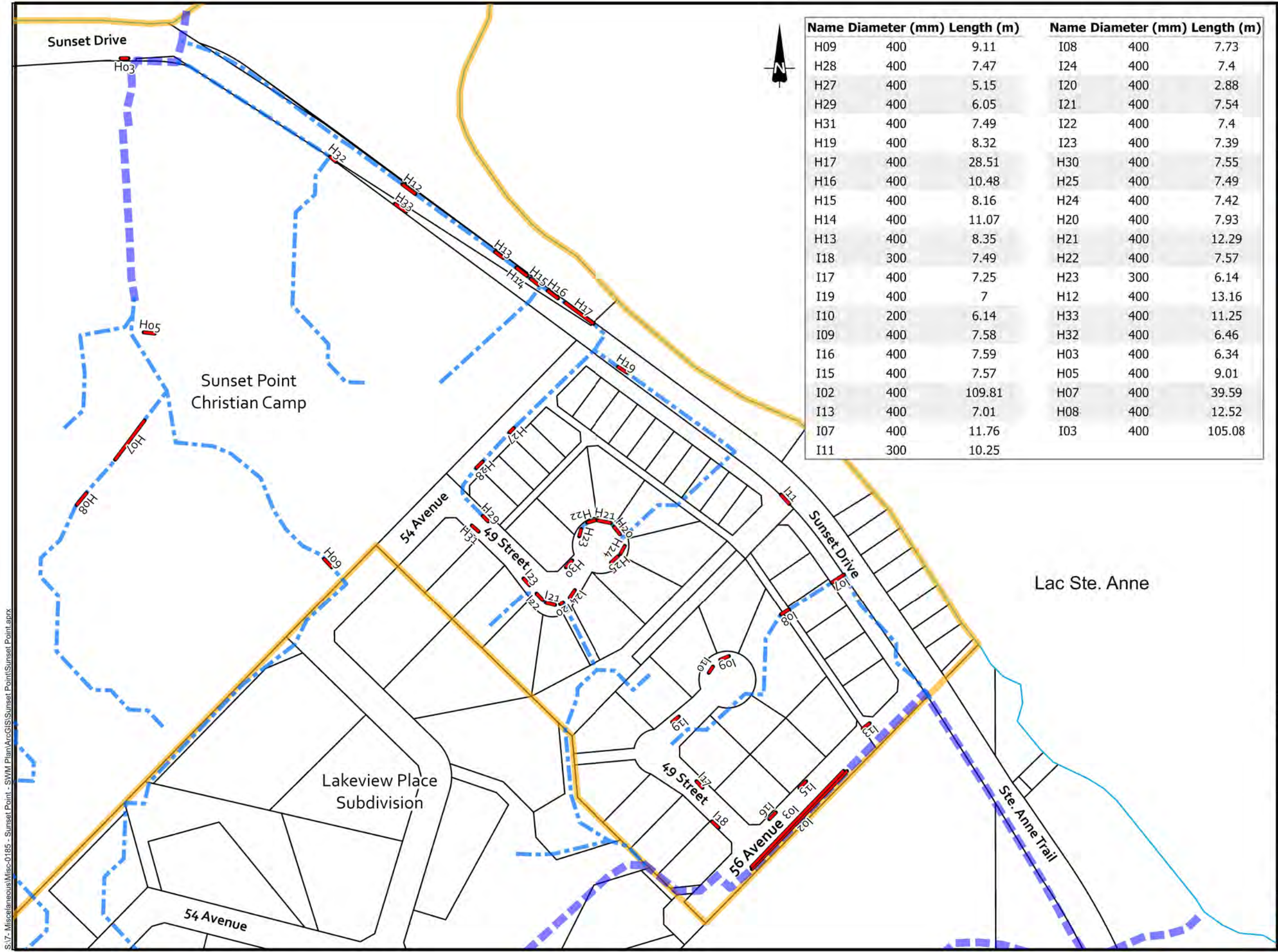
Figure 17 Undersized Culverts - 2/2
