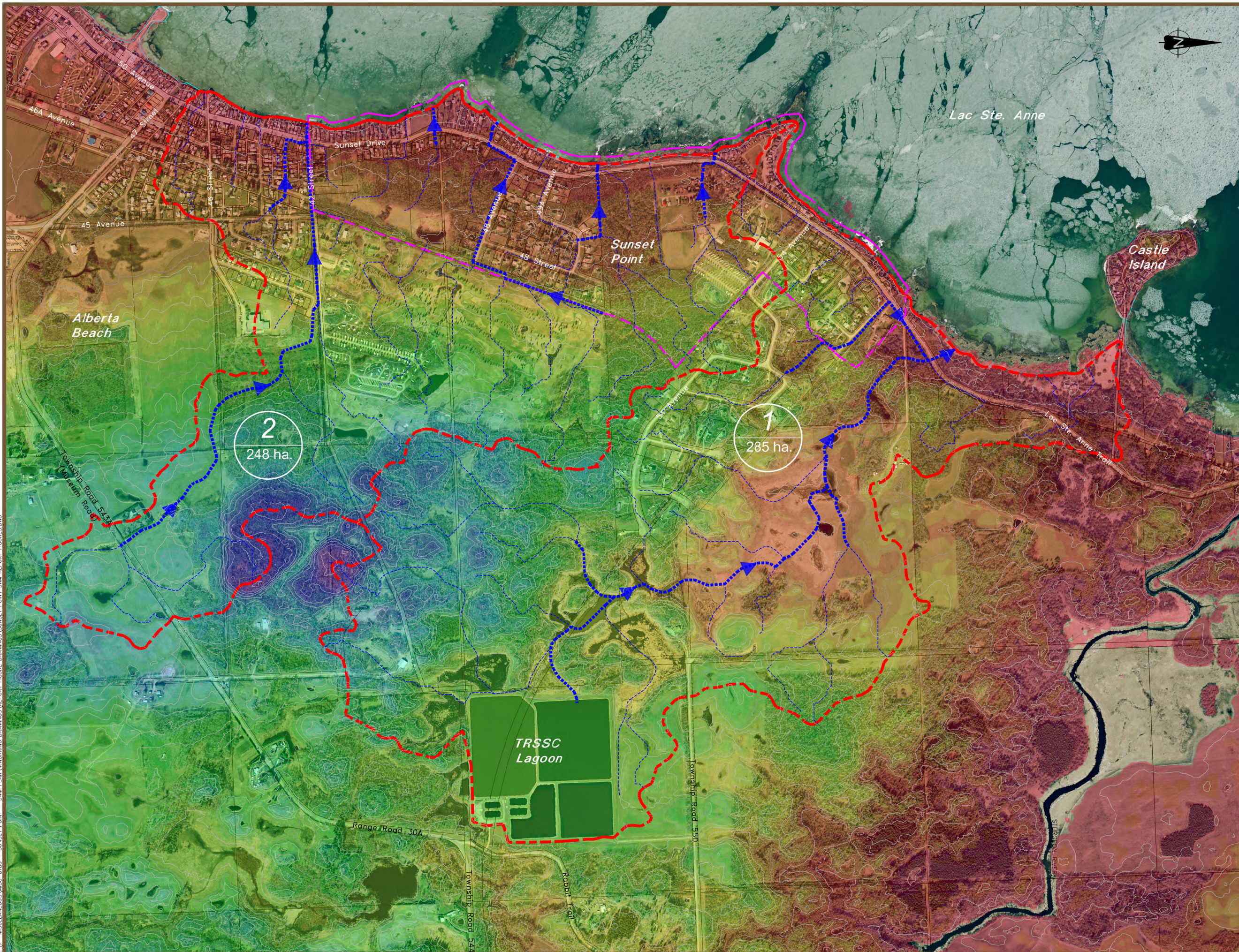
Figure 5 Regional Drainage Patterns
