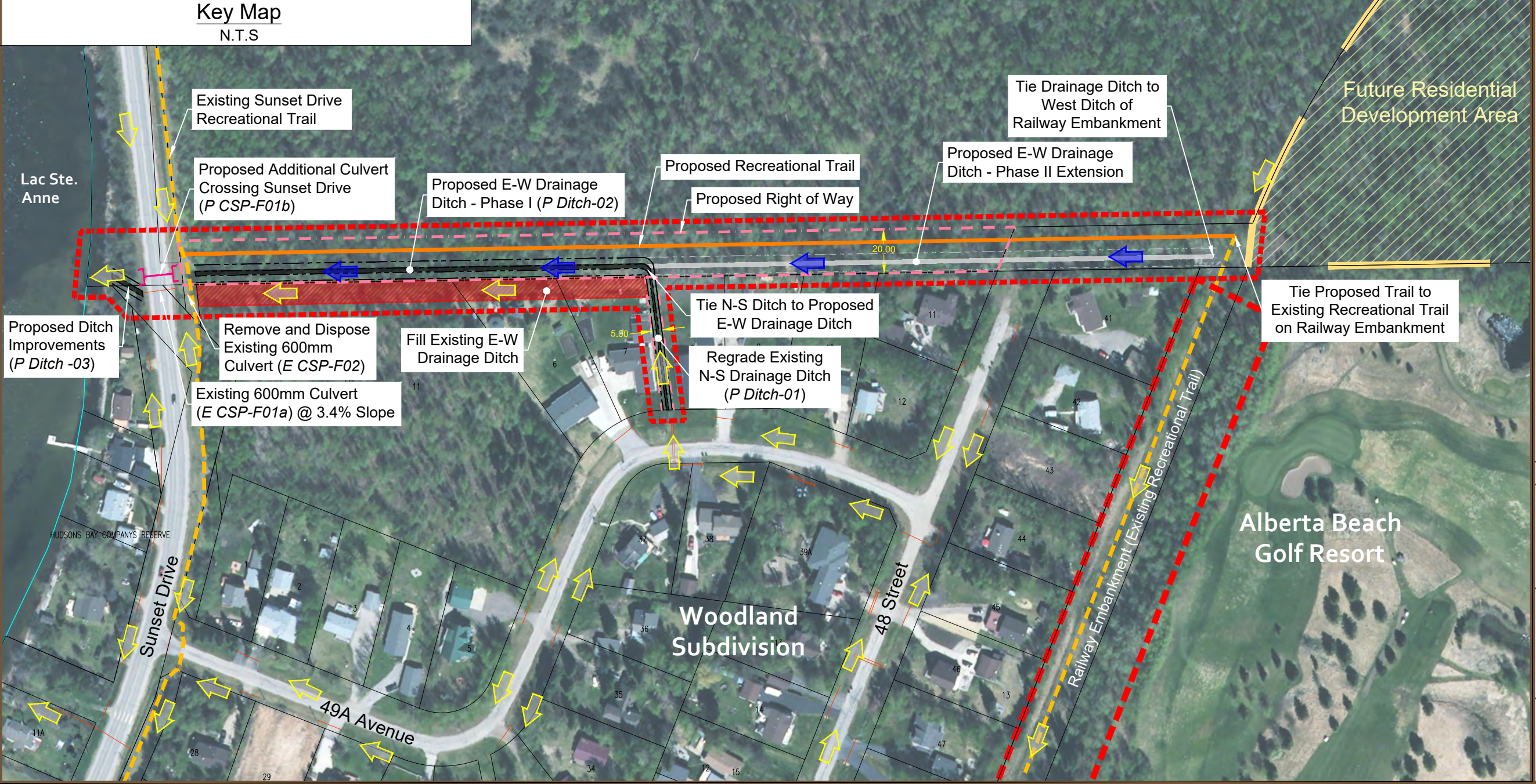
Figure 11 Project 2: Central Drainage Way
